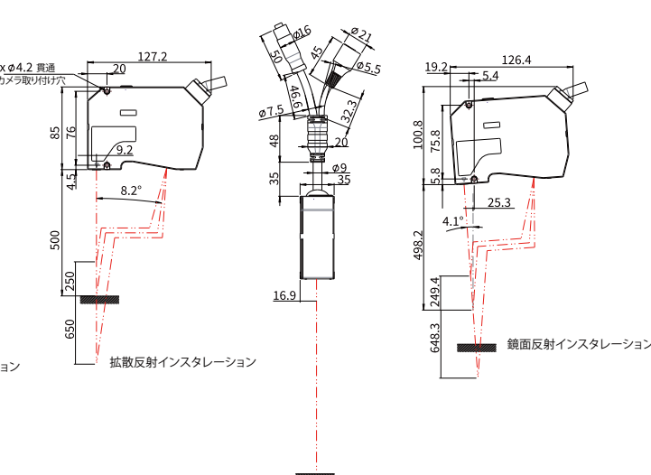
SGI500 SGI505
