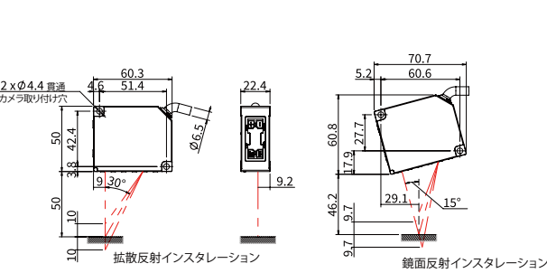
SD33-50-485-□-△
