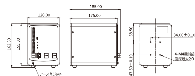
SCI502A/SCI502B one-to-two
